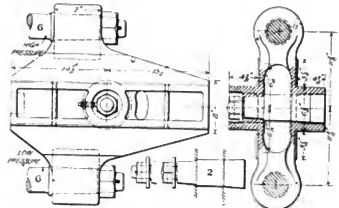
Figs. 1084-1086. Crosshead for Vaucain Compound Locomotive. Baldwin Locomotive Works.
